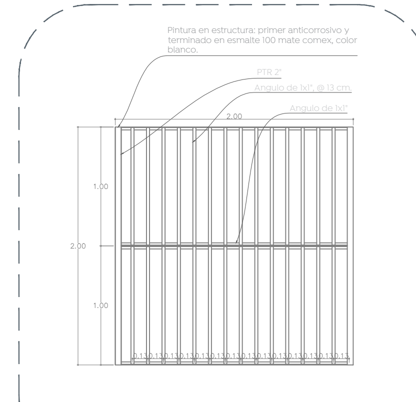
04 DET-A-02
